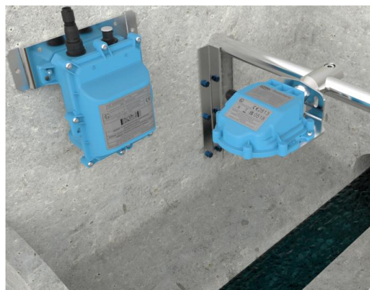
Figure 8. Bracket mount solution
