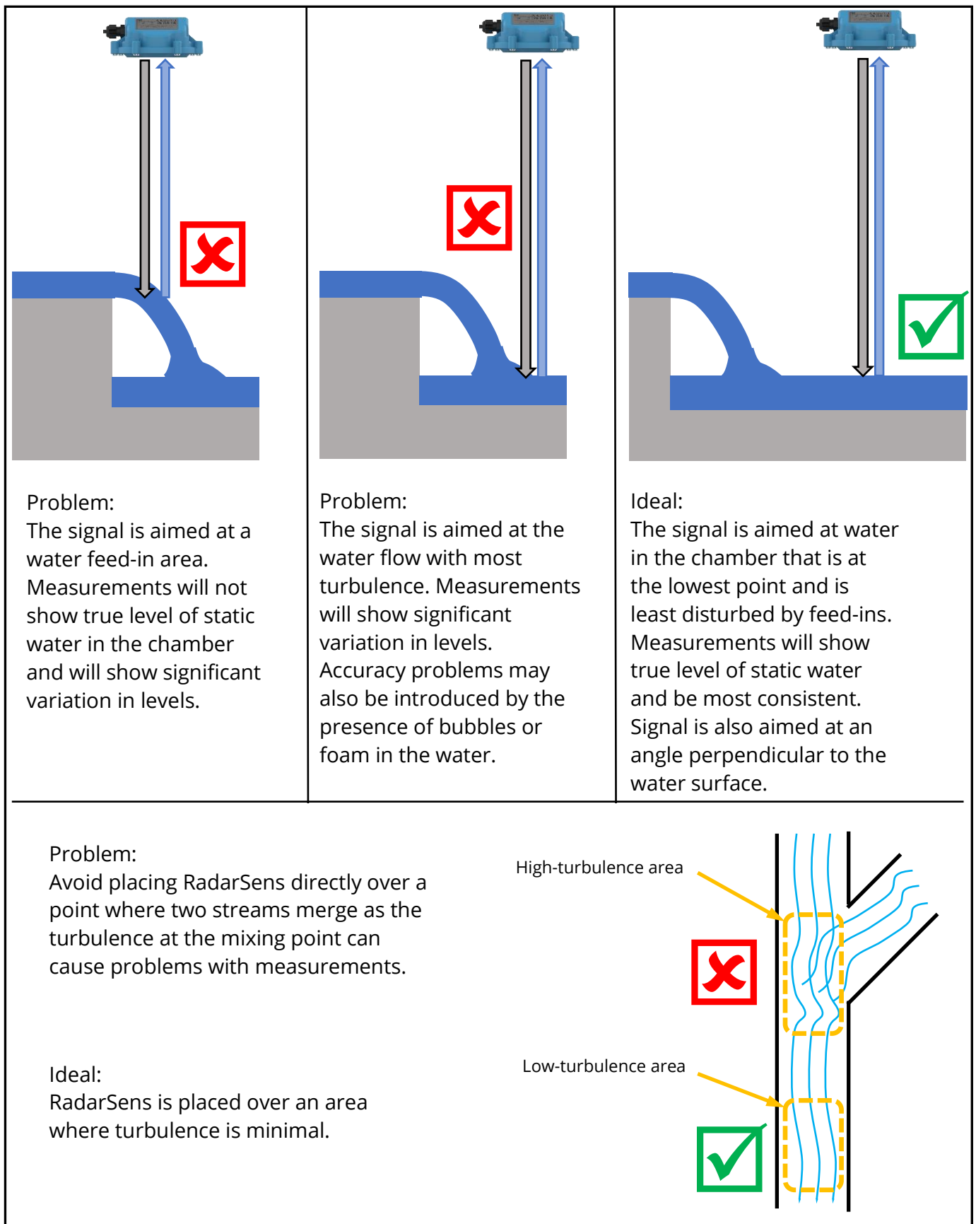
Figure 5. Turbulence avoidance
